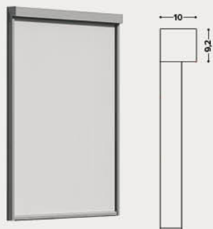
CLICK ZIP 9
